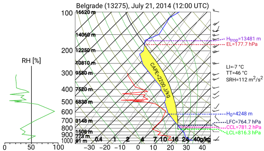
Figure 3.19 Skew-T - logP diagram for the radiosonde weather station in Belgrade (ID: 13275, Košutnjak, Lat 44^{\circ}46'15.33''\text{ N} and Lon 20^{\circ}25'29.28''\text{ E} , see Figure 3.17c) on July 21, 2014 at 12:00 UTC. The full blue and red lines are the vertical profiles of temperature and dew point, respectively. The dashed color lines represent the heights of important levels. The chart on the left and the full green line show the vertical profile of relative humidity.
