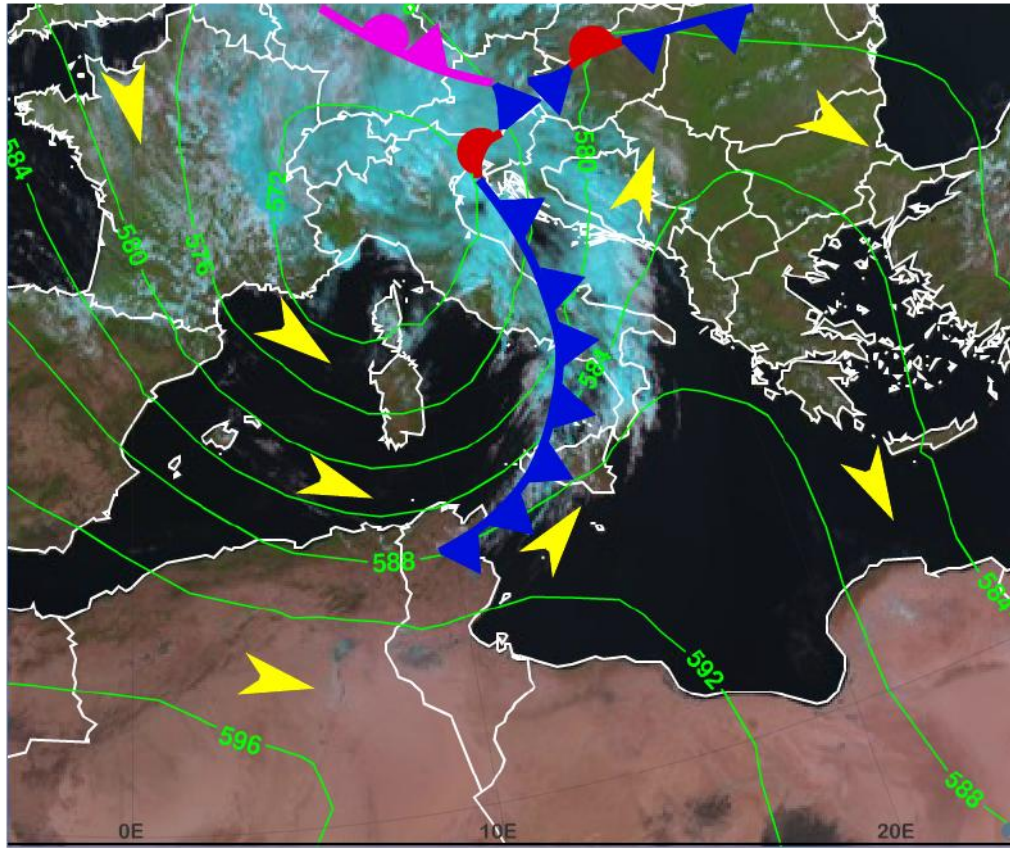
Figure 3.18 Synoptic chart of the parts of Europe and north Africa on July 21, 2014 (12:00 UTC) based on the Meteosat Second Generation satellite imagery obtained using the Natural Colour RGB channel (operated by EUMETSAT: http://www.eumetrain.org/ ). The emphasis is on the cold front above central Mediterranean and the associated cloud system. The flow direction at 500 hPa and the height of this isobaric surface in decameters are indicated with yellow arrows and green contours, respectively.
