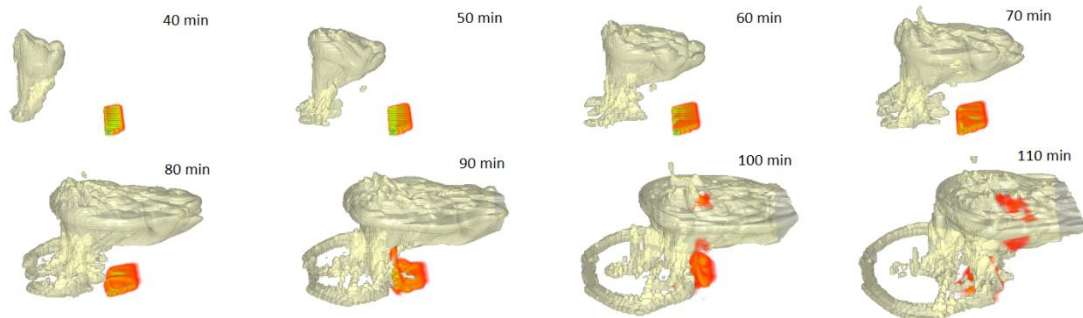
Figure 5.11 Development of the supercell cloud (grey color is cloud fraction isoline value 0.3), and transport and spreading of seeding material as passive substance.
