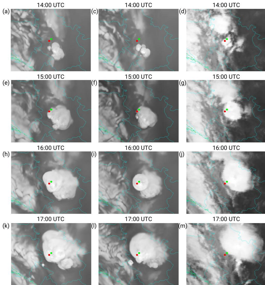
Figure 3.21 Development of supercells above Serbia according to WRF-AE (left panels), WRF-AI (middle panels) and satellite observations (right panels) from the SEVIRI 10.8 \mu\text{m} channel on board the Meteosat Second Generation satellites. The red dots are Čačak and the green dots are Gornji Milanovac. Figure 3.22 further shows that models missed the zone of pronounced radar reflectivity in the Valjevo region. Both models inaccurately predicted the location of strongest composite reflectivity around Ivanjica, instead of Čačak. Moreover, the maximum reflectivity in the modelled cases are less than 50 dBZ, which is some 10 dBZ below the observed values. Additionally, the modelled reflectivities below approximately 40 dBZ spread over the larger area compared
