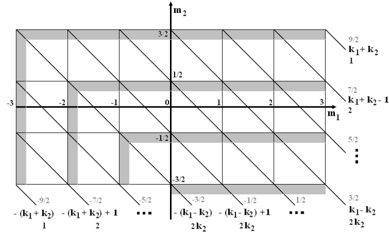
Figure 4.2: Decomposition of the product of irreducible subspaces of angular momentum. Case k_1 = 3 and k_2 = 3/2 is illustrated. At the end of each inclined line the sum m_1 + m_2 for the point (m_1, m_2) on it is depicted (concrete example is given above in gray) and the number of these points (degeneracy of the sum value) is below. Values of m_1 + m_2 included in the irreducible subspace with fixed maximal weight (written on the right side of diagram) are the lines crossed by the shaded region corresponding to maximal weight.
