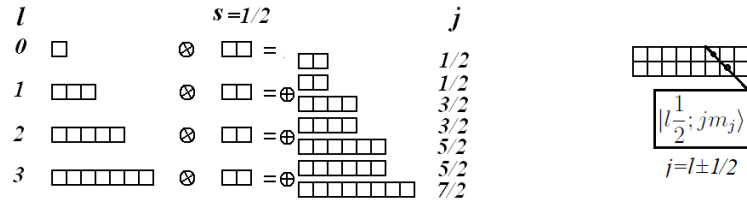
Figure 4.3: Total angular momentum of electron.
