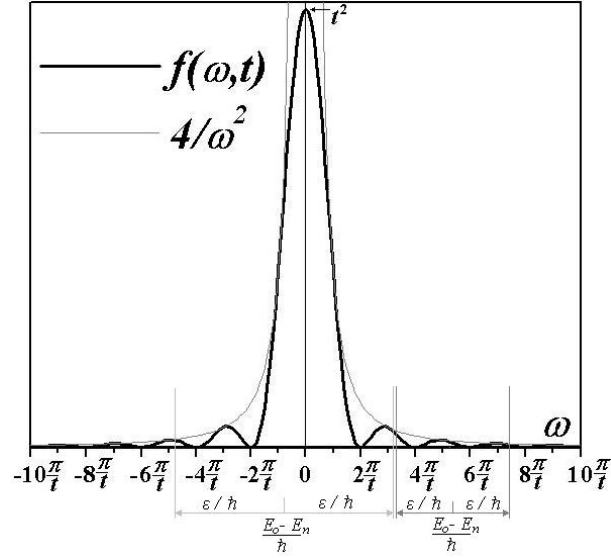
Figure 6.2: Function f(\omega, t) : note its periodicity of 2\pi/t dumped by the enveloping function 4/\omega^2 . Below: intervals of frequency corresponding to Eqns. (6.63) and (6.62).
